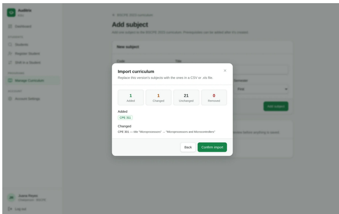
Figure 4.70. Import Curriculum – preview of changes
