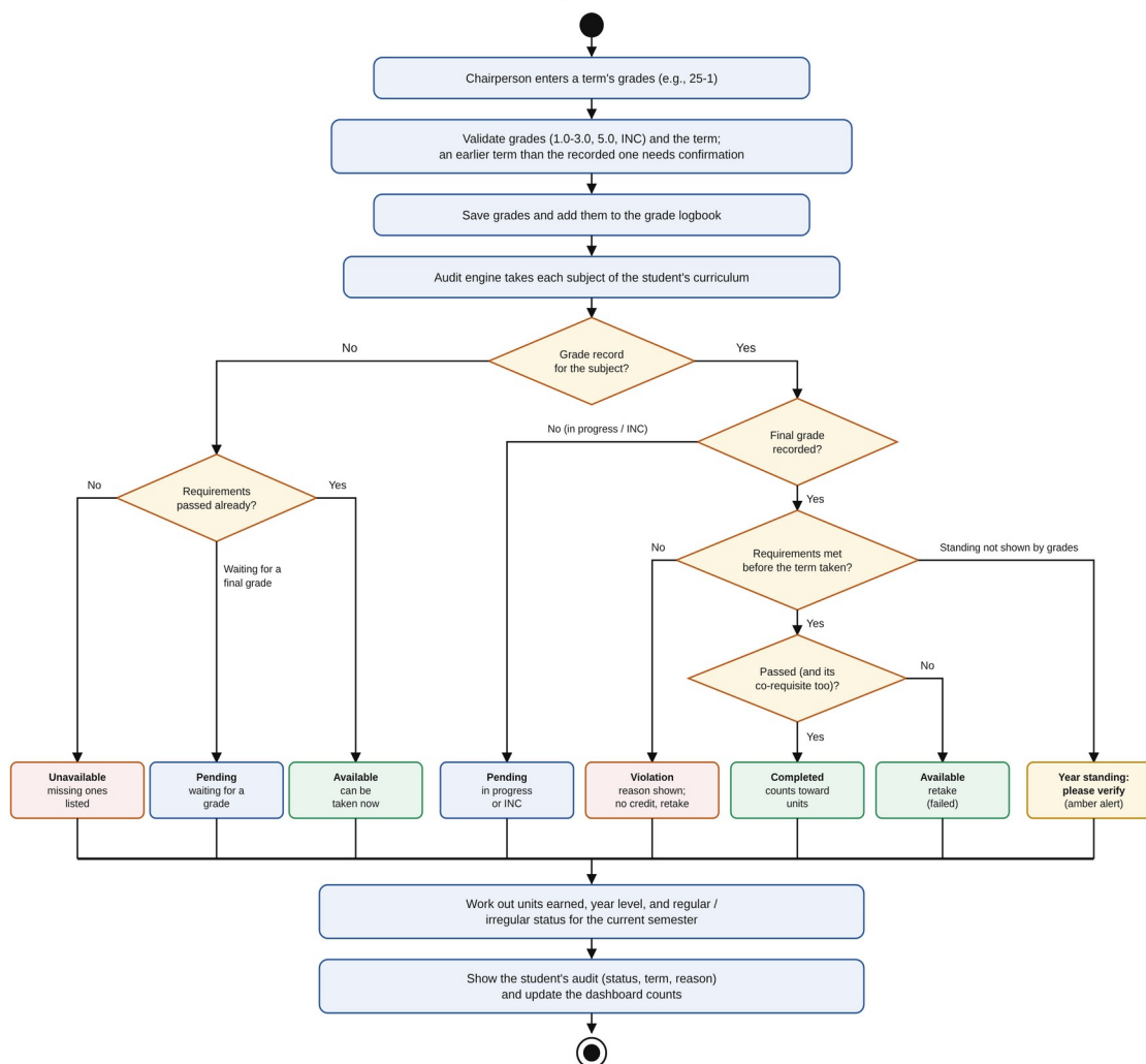
Figure 4.5. Activity Diagram of the Audit of a Subject
